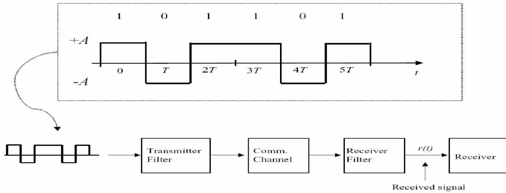
Gambar 4.8 Transmisi baseband
